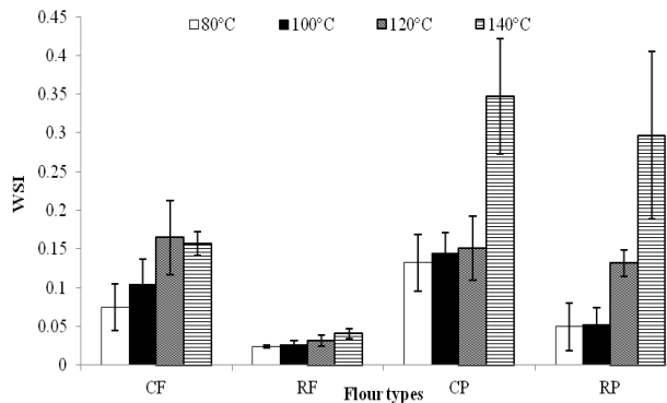
Figure 3. Water solubility index (WSI) of corn flour (CF), rice flour (RF), corn flour mixed with potato starch, 70:30 (CP), and rice flour mixed with potato starch, 70:30 (RP) at different barrel temperatures
